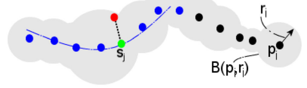
Figure 6: Variable offset ball radii and hole-filling . The offset radii r_i are adapted to changes in sample density. Simple holes are filled by projecting sample s_j from its grid location (red) in the bridging offset band onto the approximated surface (blue curve) generated by adaptive MLS (Figure 5).
